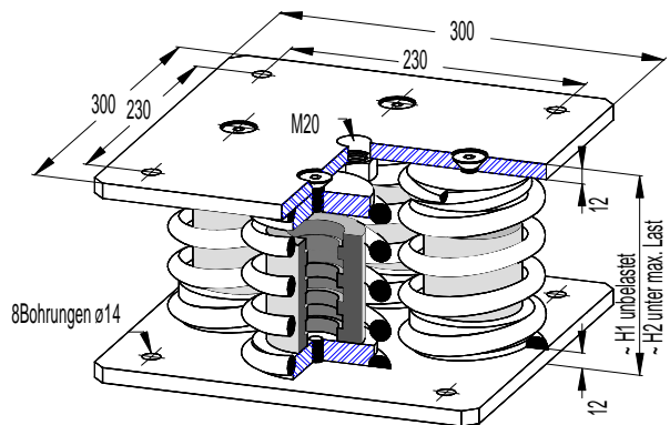
Federisolator FM-40-[ ]
