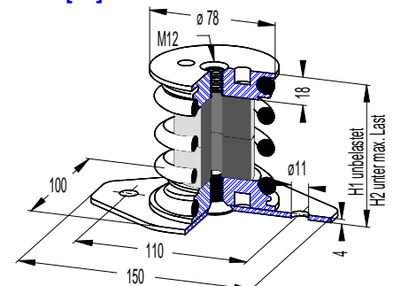
Federisolator FM-0X-[ ] C
