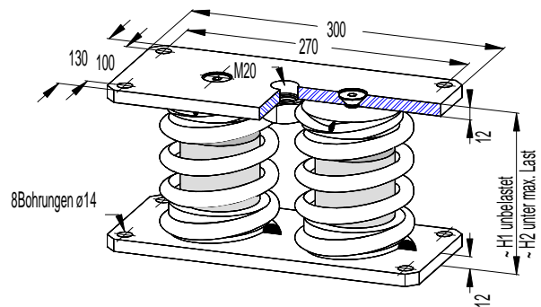
Federisolator FM-20-[ ]
