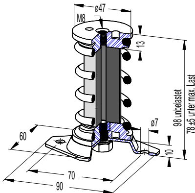
Federisolator FM-0X-341 A
