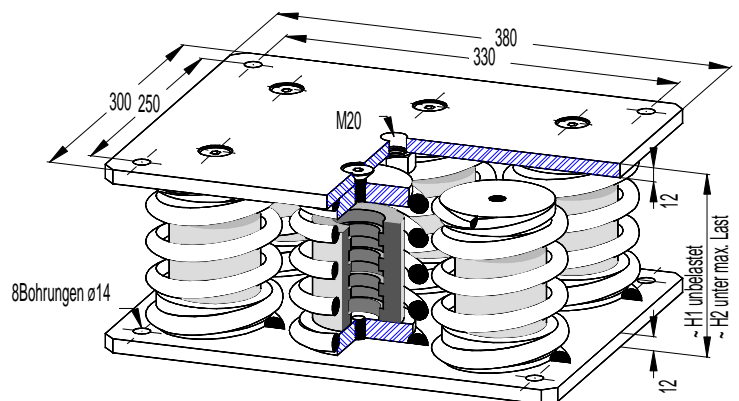
Federisolator FM-60-[ ]
