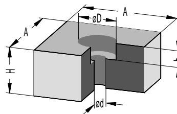
Metallkissen MQA- [ ]
